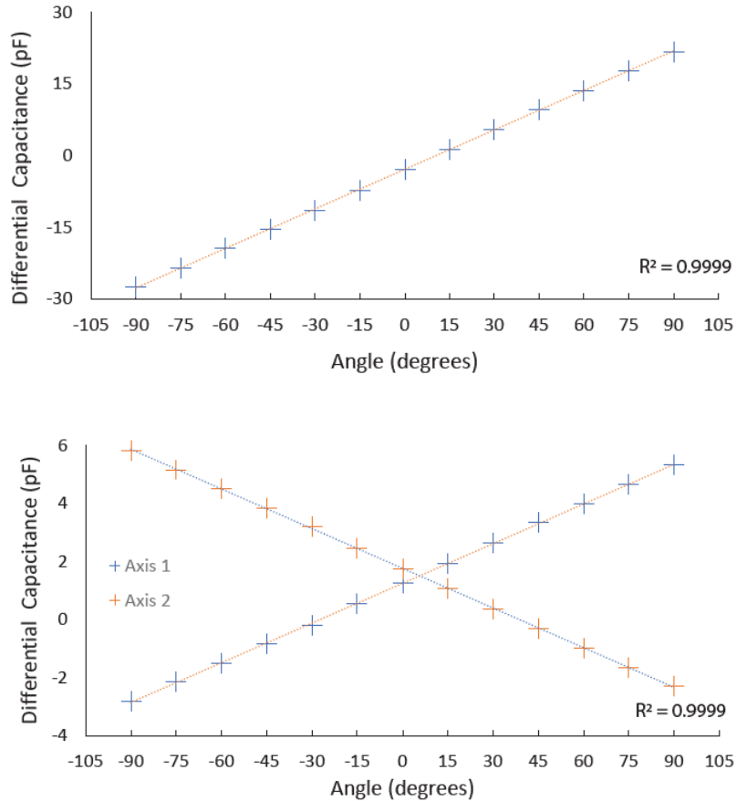
Fig 4, Sensor Linearity. (Top) A plot of differential capacitance vs. angular displacement for a one axis sensor is shown. (Bottom) A plot of differential capacitance vs. angular displacement for a both axes of a two axis sensor is shown.
